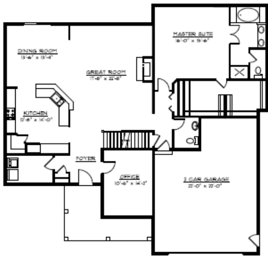
FIRST FLOOR PLAN SUMMERFIELD MODEL
