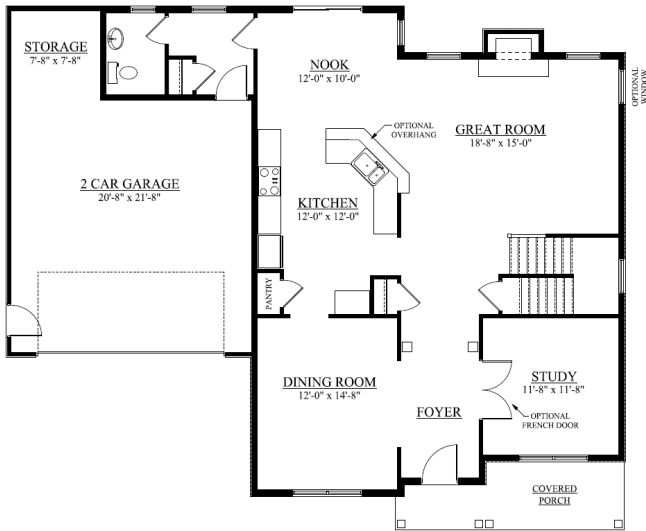
FIRST FLOOR PLAN PARKSIDE MODEL
