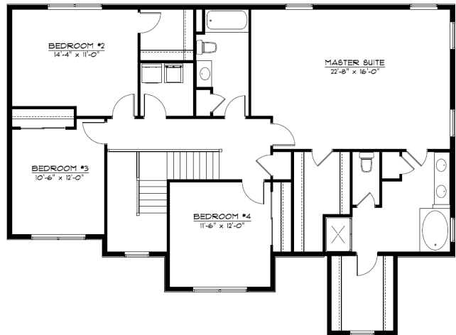
SECOND FLOOR PLAN FAIRVIEW 3 MODEL
